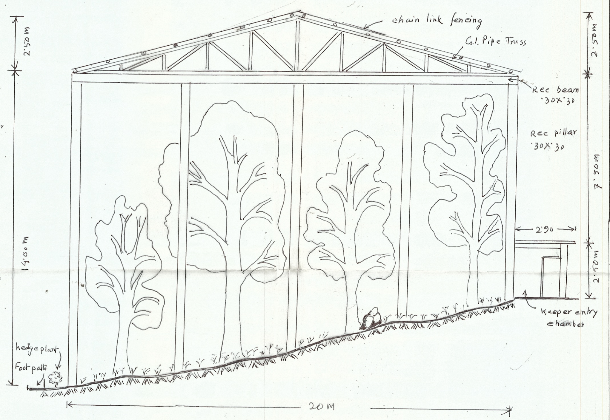
ENCLOSURE SECTION
