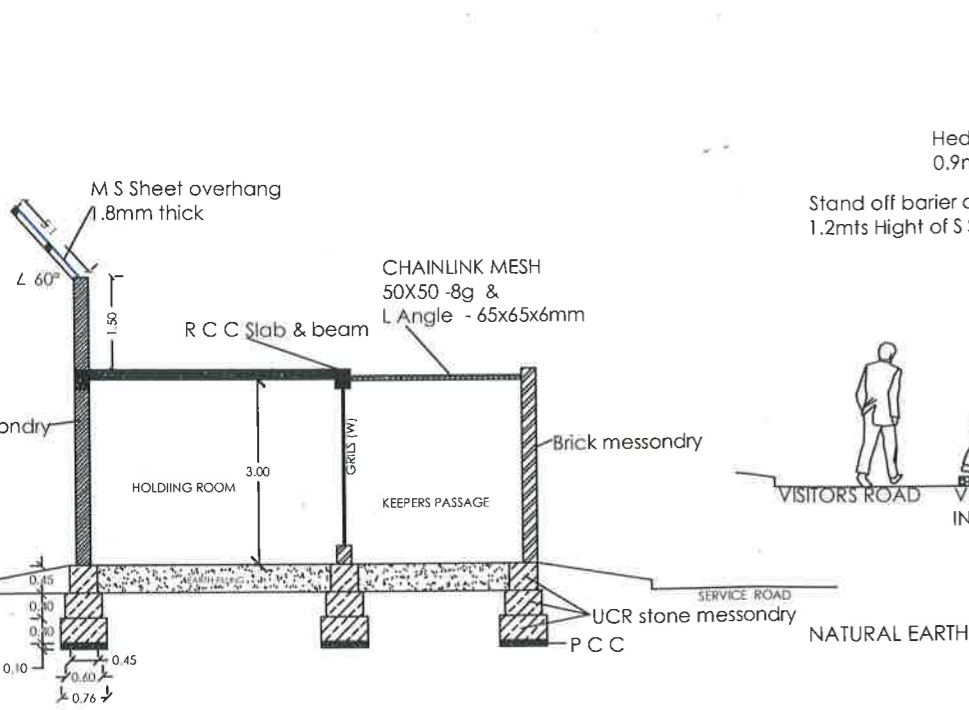
SECTION @ BB
