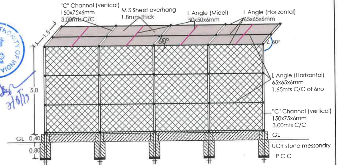
ELEVATION OF OUTER FENCING
