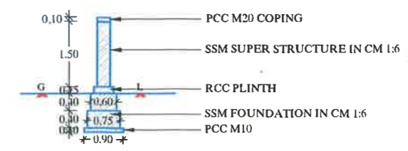
CROSS SECTION OF HOLDING ROOM WALL
