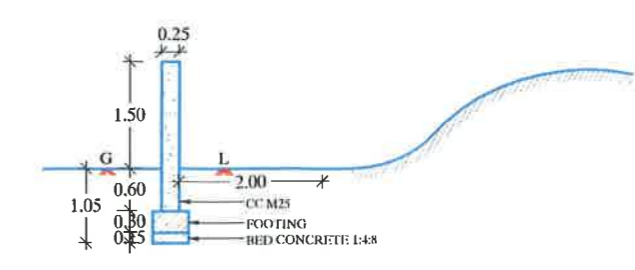
CROSS SECTION OF MOAT WALL
