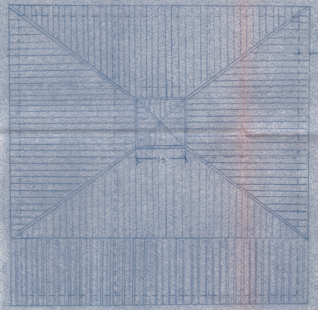
ROOF PLAN
