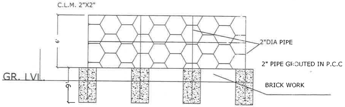
ELEVATION OF KRAAL FACILITY
